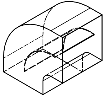
Rectangular Radius Bend with Turning Vanes
